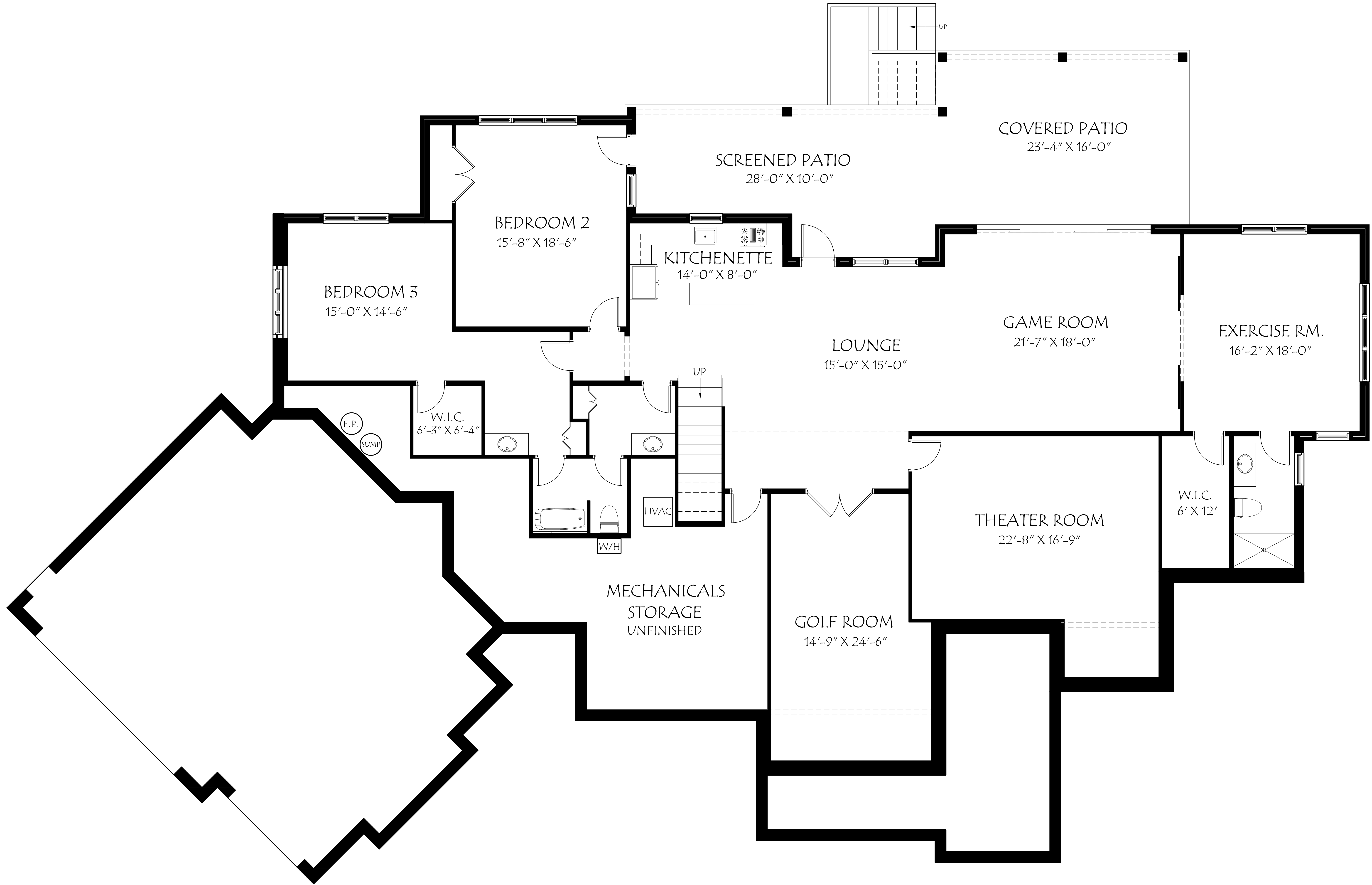
PROPOSED LOWER FLOOR PLAN
